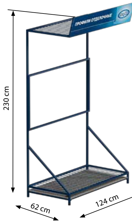
Stand for profiles 52/20 Decoplast LUX (Ecoline skirting)
