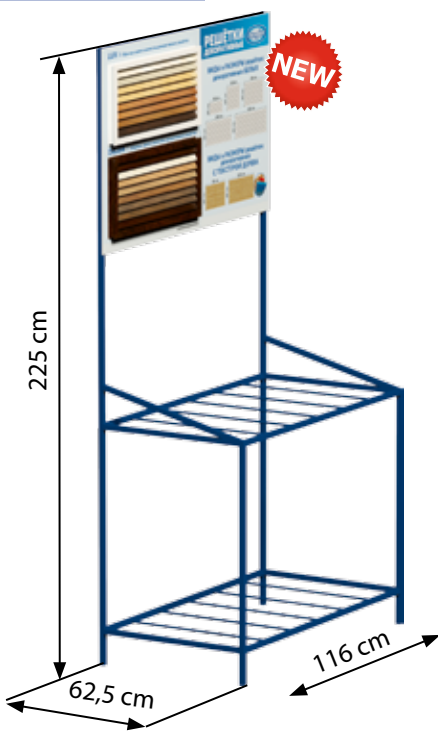
Stand for decorative screens Decoplast LUX
