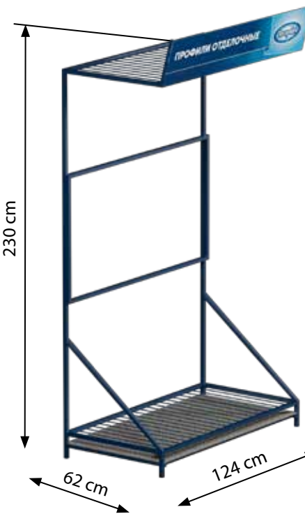
Stand for profiles 60/17 Decoplast LUX (skirting 60, door trim)
