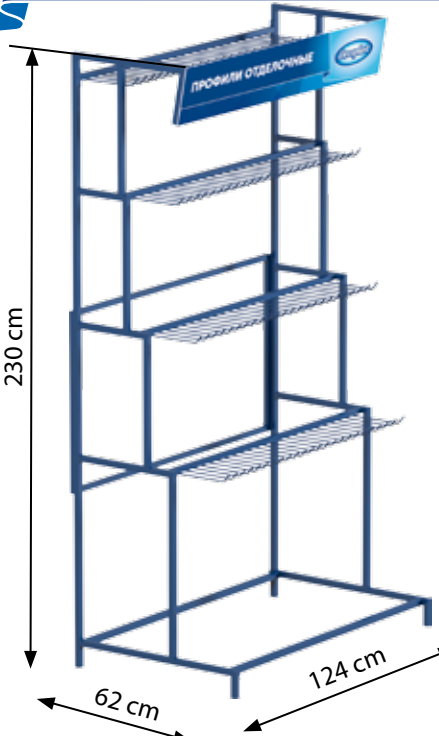
Stand for doorsills 4/96 Decoplast LUX
