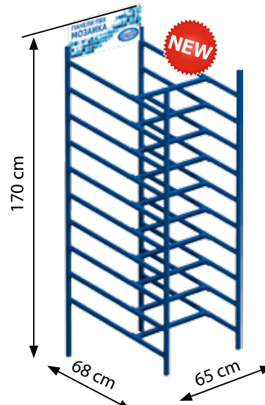
Stand for mosaic PVC Decoplast LUX
